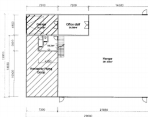
Ground Floor Scale 1/200
