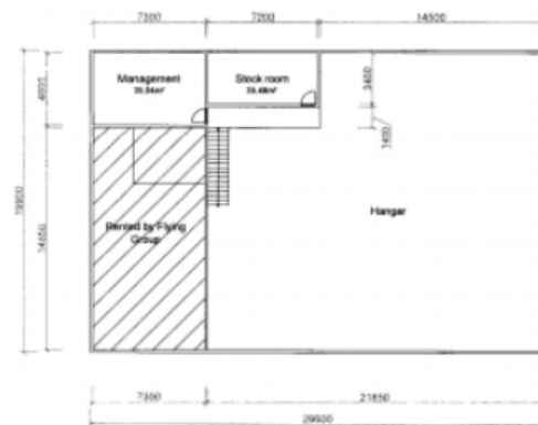
First Floor Scale 1/200
